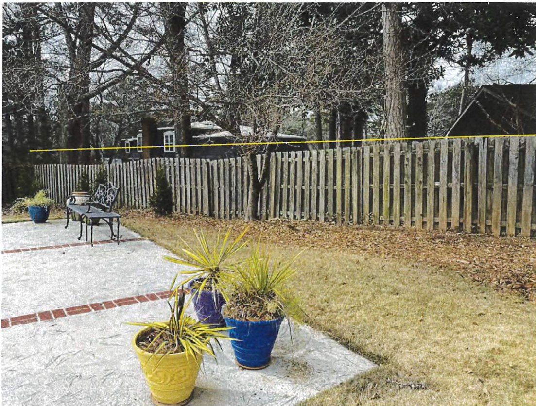
Above: View looking approximately West toward the houses on Lakeview Plaza. Line shows change from a 6' height on the right, gradually increasing to 8' at the far left. Below: View looking along the NW edge looking approximately NW toward the houses on Lakeview Plaza. Line shows stepped height starting at 6' at the left, increasing to 8' approaching the corner at the bottom of the grade.
